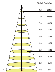
Beam Angle(B): 109.1 V75.9 Field Angle(F): 113.5 V128.1
