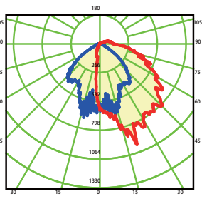
Average Diffuse Angle(50%): 87.0° Unit: cd — C0-C180 — C90-C270
